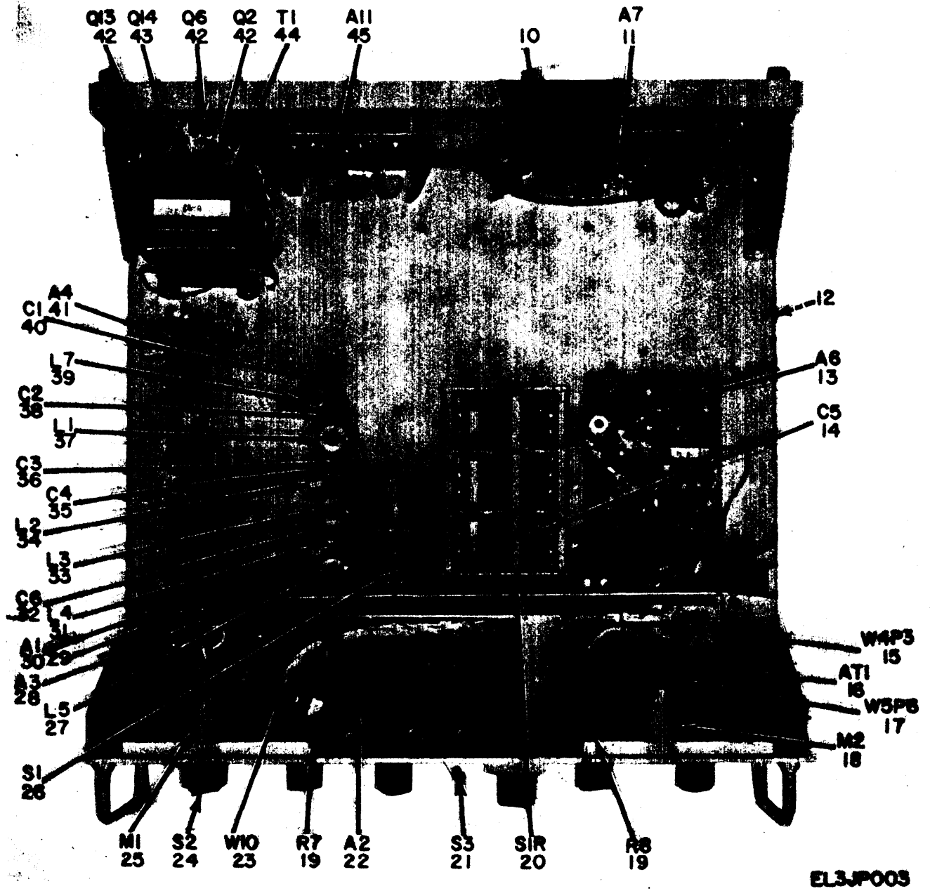
Figure 2. Generator, Signal SG-479C/GRM-50 (Sheet 2 of 3).
