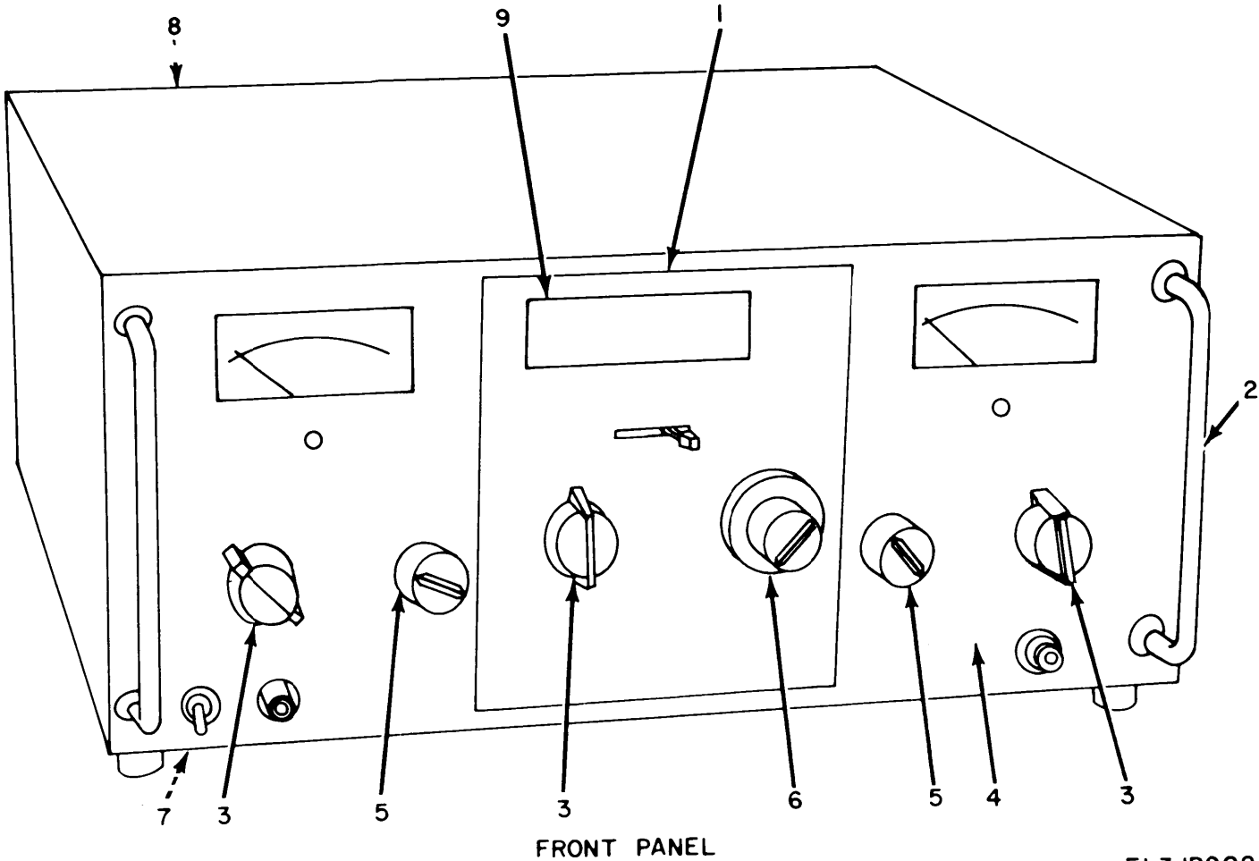
Figure 2. Generator, Signal SG-479C/GRI1-50 (Sheet 1 of 3).
